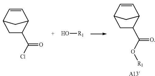
&lt;Reaction Scheme 2&gt;
