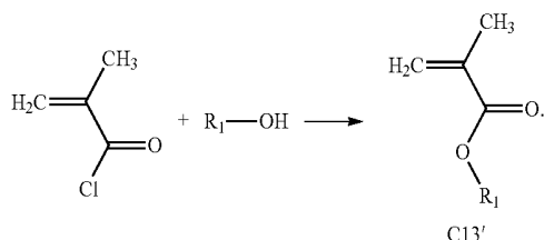
&lt;Reaction Scheme 3&gt;
