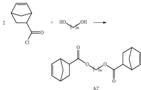
&lt;Reaction Scheme 4&gt;
