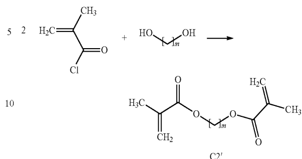
&lt;Reaction Scheme 5&gt;
